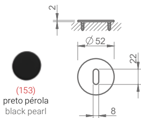
Key entry set European cylinder entry
